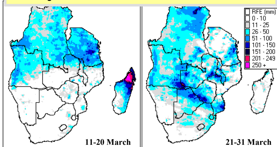
Fig.1. Rainfall Performance for 11 to 31 March 2007
