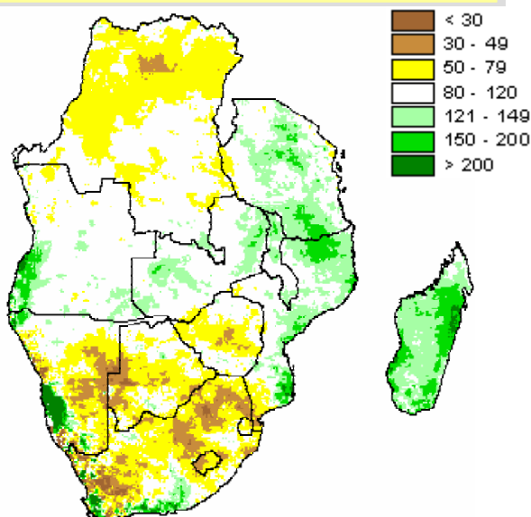
Fig.2. Rainfall for 1 Jan to 31 Mar 2007 as Percentage of Normal
