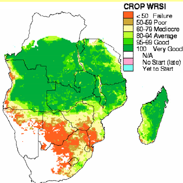
Fig.3. Water Requirements Satisfaction Index as at 31 March 2007
