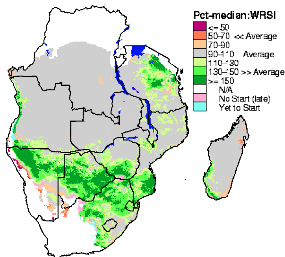
Figure 3. WRSI expressed as a percentage of normal conditions. Source: USGS/FEWSNET
