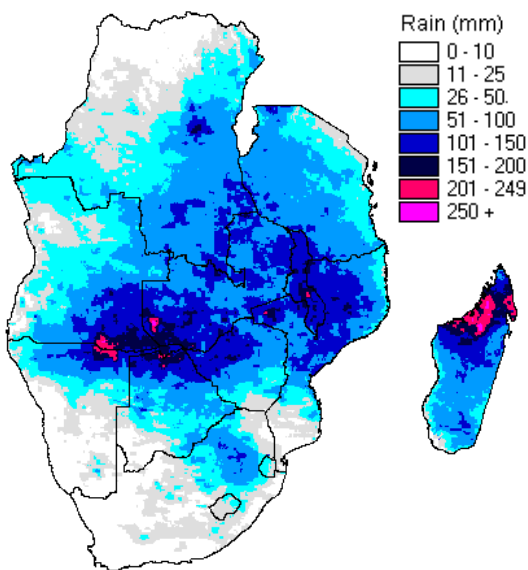
Figure 1. Rainfall for 21-31 January 2008, from rainfall estimates (data source: NOAA/FEWSNET)
