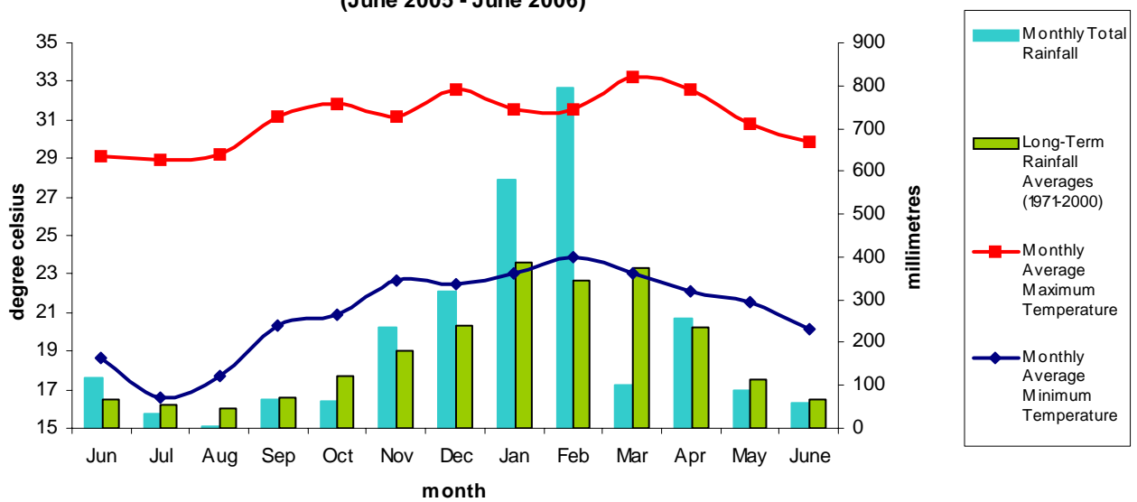
Labasa Airfield - Temperature & Rainfall Records for the last 13 Months (June 2005 - June 2006)
